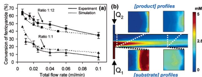
Figure 2. (a) Conversion of ferricyanide to ferrocyanide as a function of the flow rate at flow rate ratios Q_2/Q_1 of 1 and 12. (b) FEMLAB visualization of the substrate and product concentrations at the flow rate ratio Q_2/Q_1 of 1 (total flow rate of 0.01 mL/min).
