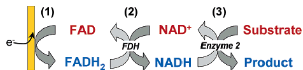
Scheme 1. Indirect Electrochemical Regeneration of NADH Using FAD/FADH 2 as the Mediator and Subsequent Biocatalytic Conversion
