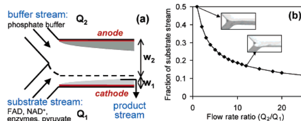
Figure 1. (a) Schematic of the electrochemical microreactor for cofactor regeneration and subsequent biocatalytic substrate conversion. In gray: reaction depletion zones (not to scale). (b) Adjustment of the width or focusing of the substrate stream by change of the ratio of volumetric flow rates, Q_2/Q_1 . Insets: optical micrographs of two differently dyed aqueous streams in laminar flow at Q_2/Q_1 = 1 and 12.
